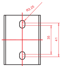
Bottom & Side Mounting
